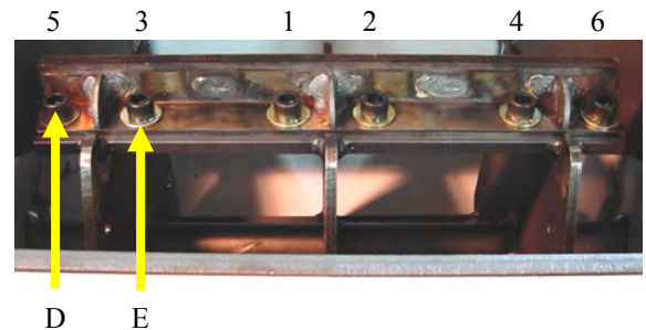
Blade Bolt Torque Sequence
